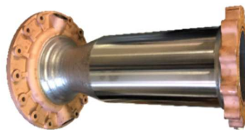
Figure 17: NASA – RDT Advanced Lander Propulsion Additive Cold Spray Assembly (ALPACA) [10].
