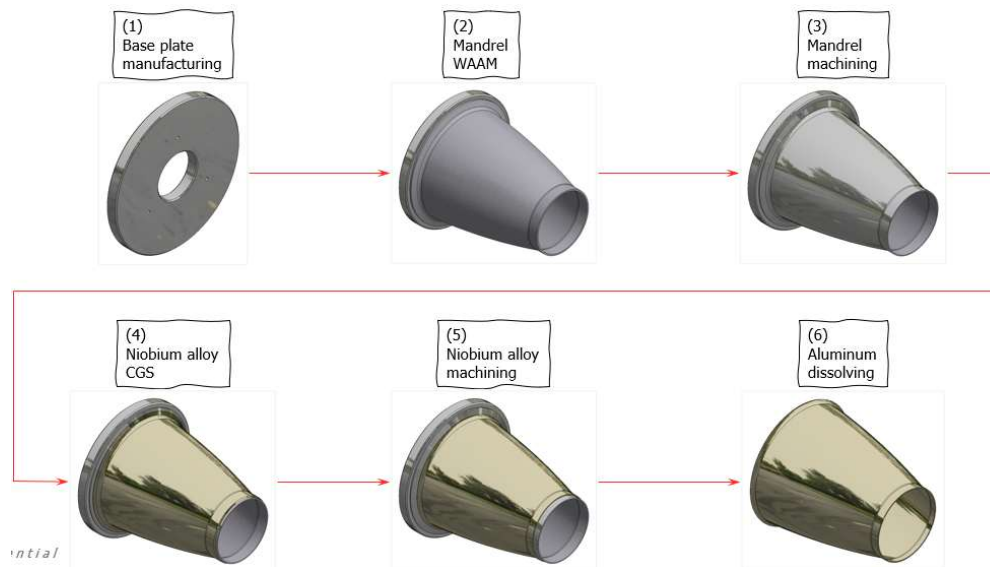
Figure 8: Schematic process flow of manufacturing a C-103 nozzle extension while using WAAM, machining, Cold Spray and mandrel removal [13].
