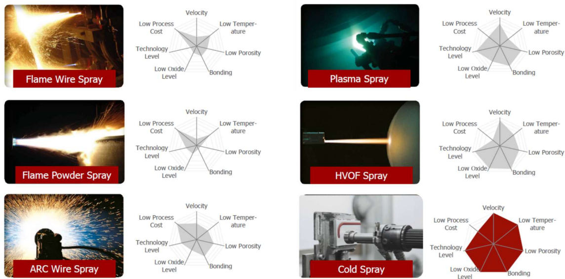
Figure 1: Cold Spray another technology in the family of thermal spray processes [4].
