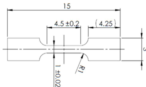
Figure 7: Geometry of cut out tensile specimen [13].
