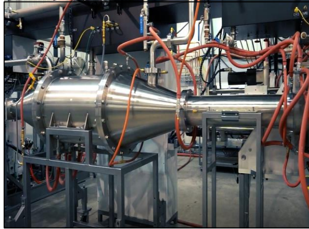
Fig 4. Supersonic Diffuser with heat exchanger
