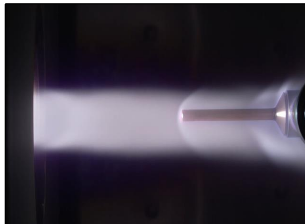
Fig 7. Tekna enthalpy probe inside the plasma plume
