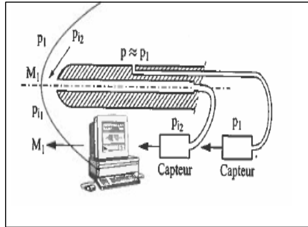
Fig 6. Tekna supersonic enthalpy probe design
