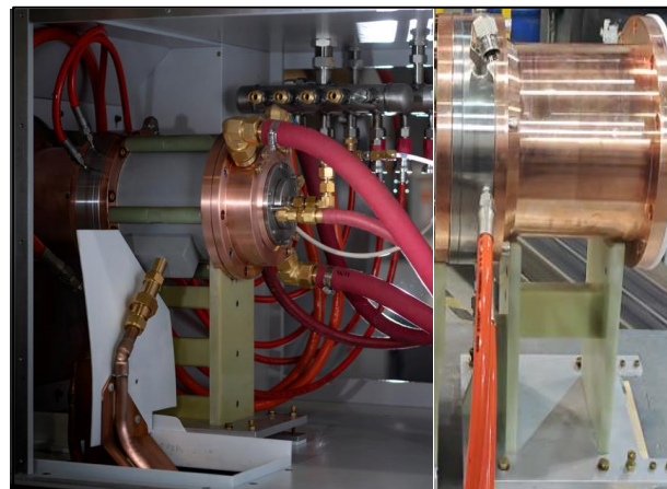
Fig 2. Tekna 350kW-ICPT torch with nozzle
