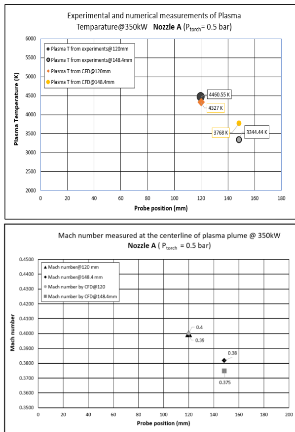
Fig 10. a) Temperature and b) Mach number calculated from Tekna enthalpy probe and CFD model.
