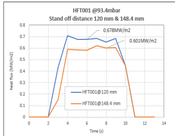
Fig 12. Heat flux measurement in MW/2 obtained experimentally.
